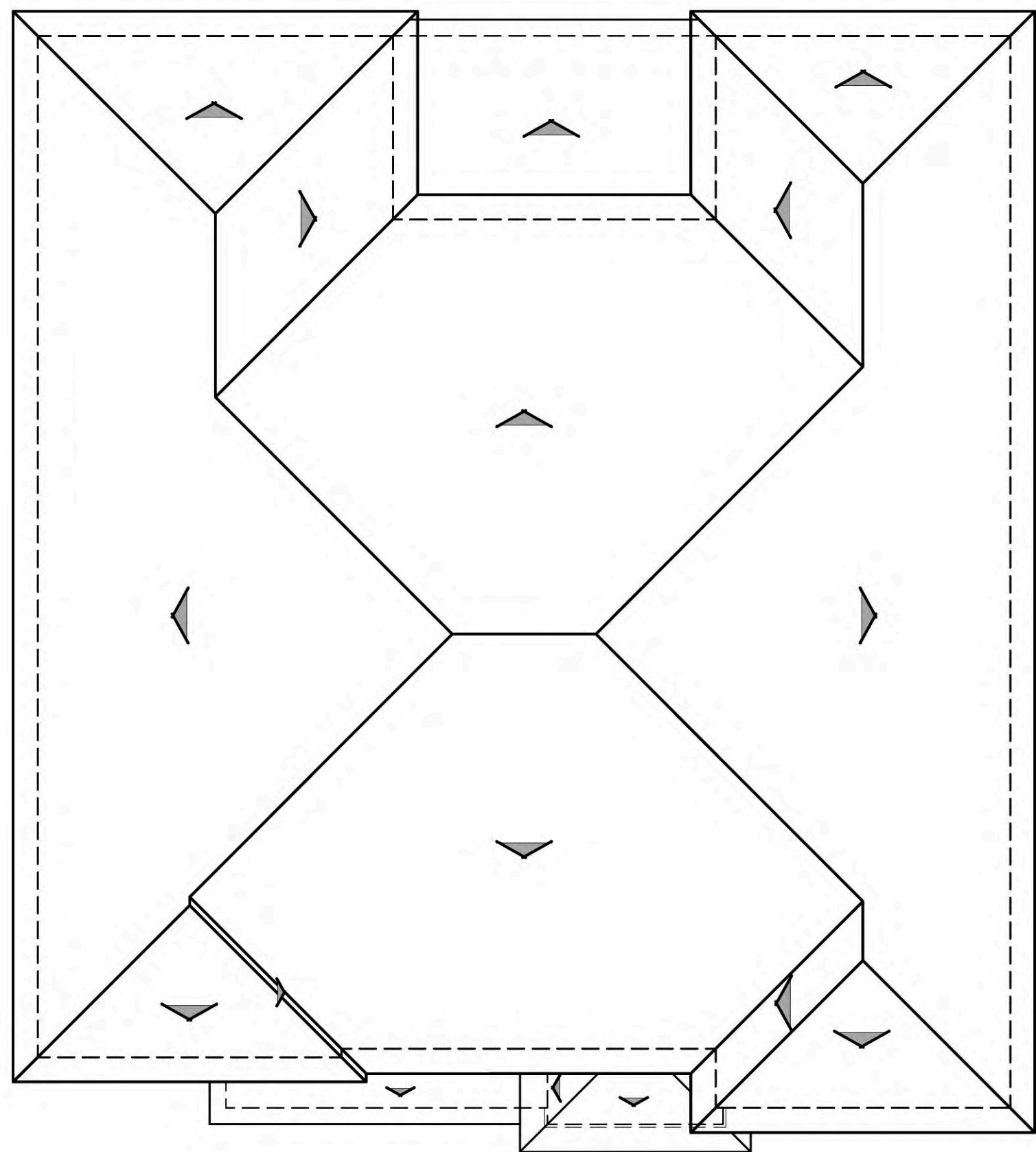
ROOF PLAN
