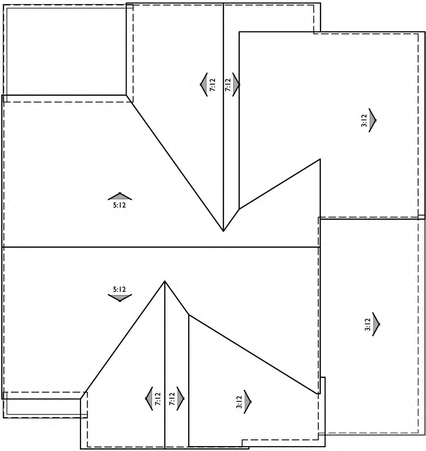
ROOF PLAN
